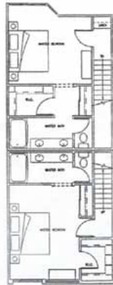
UNIT 9L/9b - 3rd Level
