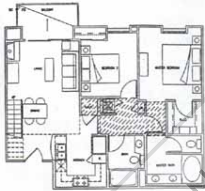
UNIT 7m - 6th Level ⑤
