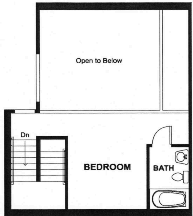
UPPER LEVEL
